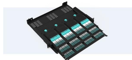
Pre-Terminated Patch Panel
