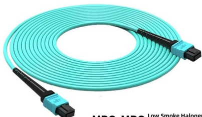
MPO-MPO Low Smoke Halogen Free Sheath Multimode 10 Gigabit 24 pole OM3 Insertion loss <0.35dB Return loss >50dB
