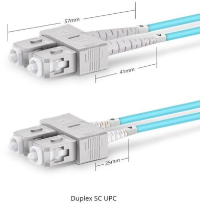
Duplex SC UPC
