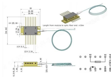
Outline drawings
