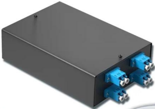
4-port 8-core LC wall-mounted fiber terminal box (empty frame) | Surface painted Scientific plate fiber Cold-rolled steel plate
